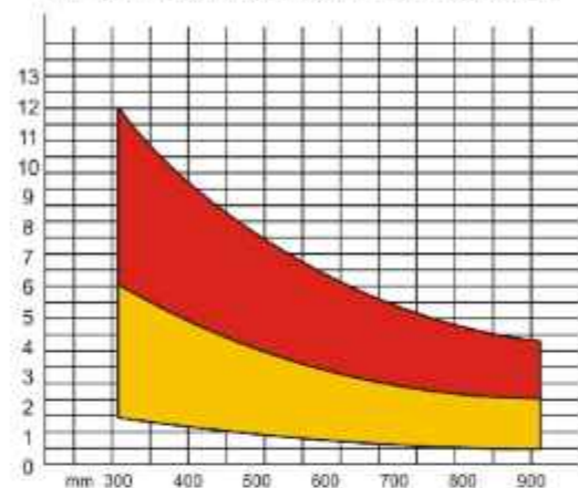
SUPPORT BEARING CAPACITY-支撑承载力说明图
