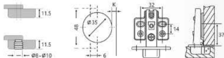
AF826 3D06 Aluminum Frame 3D Gun Black Hinge with 6 hole
