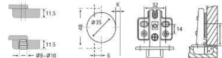
SA2 Iron Short Arm Hinge With 2D screw
