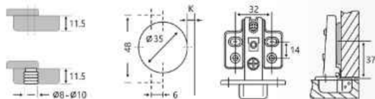
GCN863 Half SS Hydraulic Hinge
