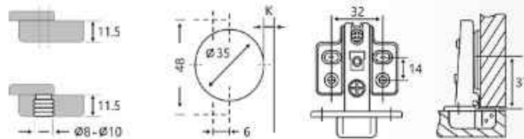
AFSS SS Hydraulic Hinge With Hook
