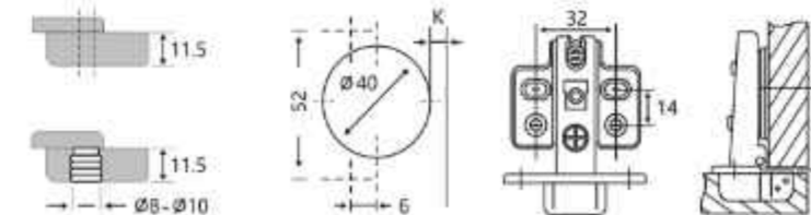
GC401 Slide-on Iron Hydraulic Hinge
