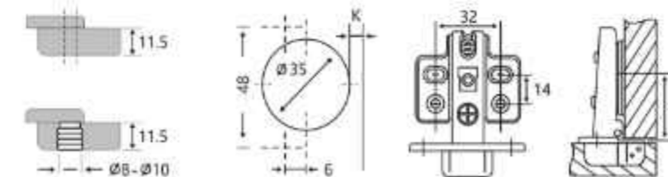
GC3D04 SS or Iron 3D Hydraulic hinge
