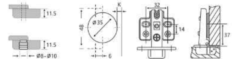
90° 3Dhinge / 90° 3D铰链
